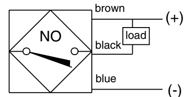
BTPX-N (NPN) (Current sinking)
