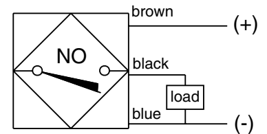
BTPX-P (PNP) (Current sourcing)
