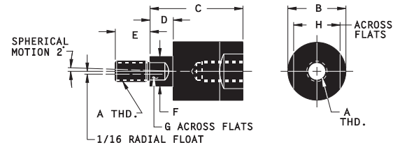
ALIGNMENT COUPLER*
