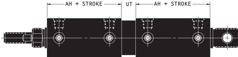
SERIES FT/DT
