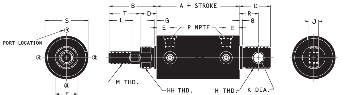
SERIES DSI/DSIM
