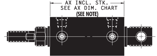
SERIES FSR/OSR/HSR/DSR CONSULT FACTORY FOR STROKES LONGER THAN 6" (10" MAX. AVAILABLE)
