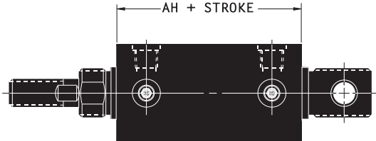
SERIES H/D
