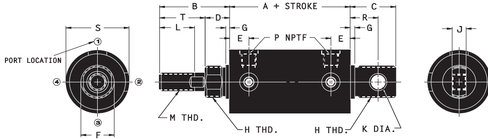
SERIES F/O/OLF
