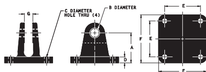
SWIVEL BRACKET
