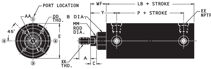
SERIES FI/OI/OILF/OIM
