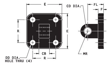
PIVOT BRACKET
