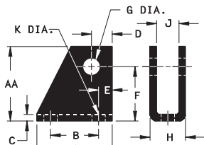
SWIVEL BRACKET
