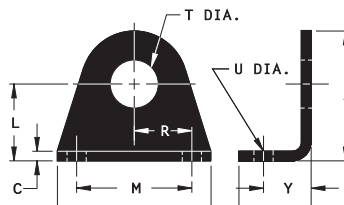
FOOT BRACKET
